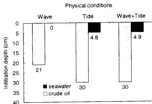
Fig. 3. Penetration depth of seawater and crude oil by wave and/or tidal actions.
