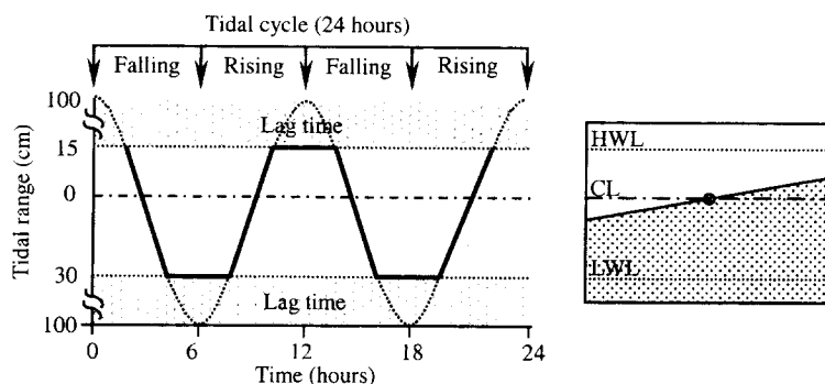
Fig. 2. Tidal fluctuation. Dashed line shows tidal range from the sediment surface of observation window on right side (HWL; high water level, CL; center line, LWL; low water level)
