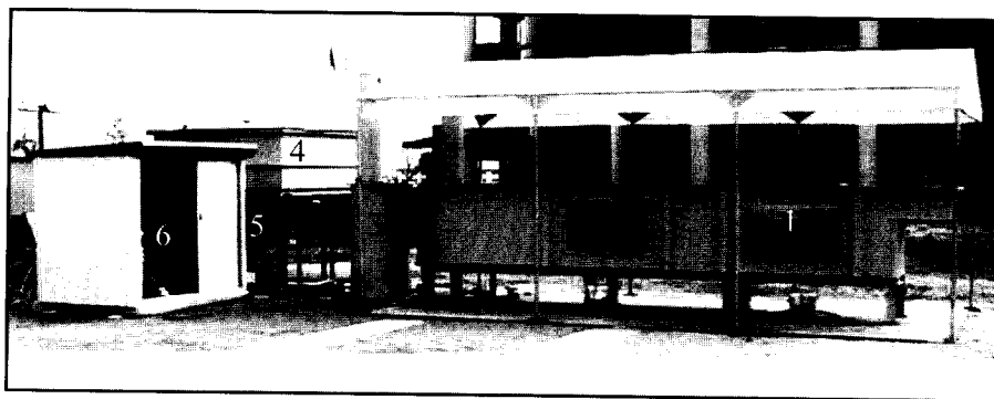
Fig. 1. Image of model sandy beach (1: sandy beach, 2: wave maker, 3: tide control device, 4: reservoir, 5: temperature control system, 6: computer control system).
