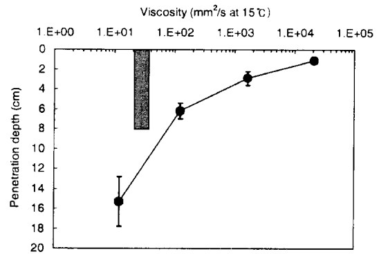
Fig. 7. Relationship between viscosity and penetration depth in the silicon oil and crude oil. Symbols show the penetration depth of the silicon oil (black circle and standard deviation) and the crude oil (gray panel) with standard deviation (error bar).
