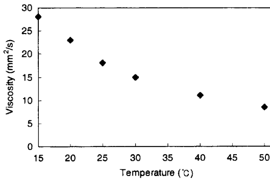
Fig. 6. Relationship between viscosity and temperature in the crude oil.
