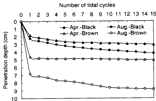
Fig. 4. Long-term penetration of the stranded crude oil into the sediments in April 20-27 and August 20-27.
